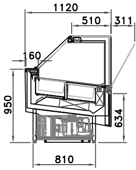
WITHOUT PANELS
