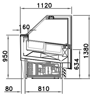
WITH PANELS
