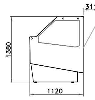
WITH PANELS
