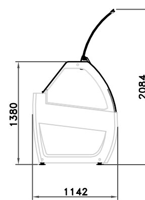
WITH PANELS
