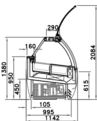
WITH PANELS
